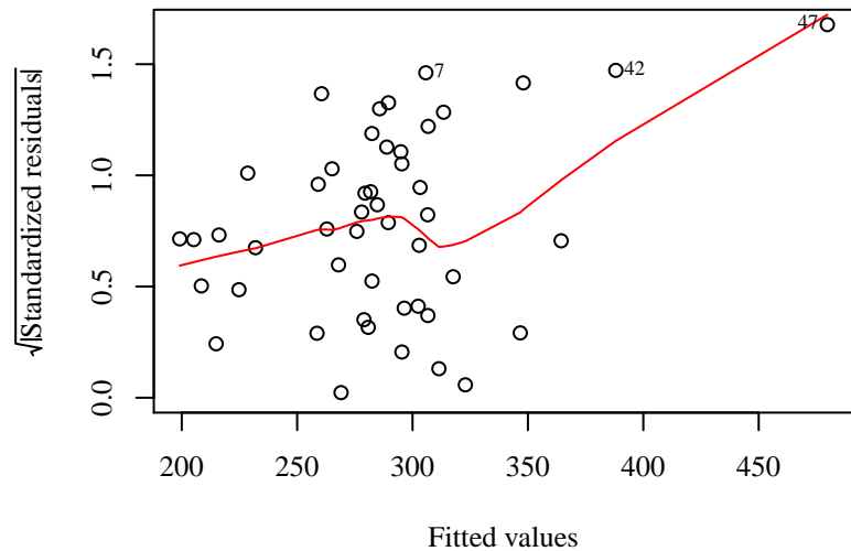
Scale-Location
