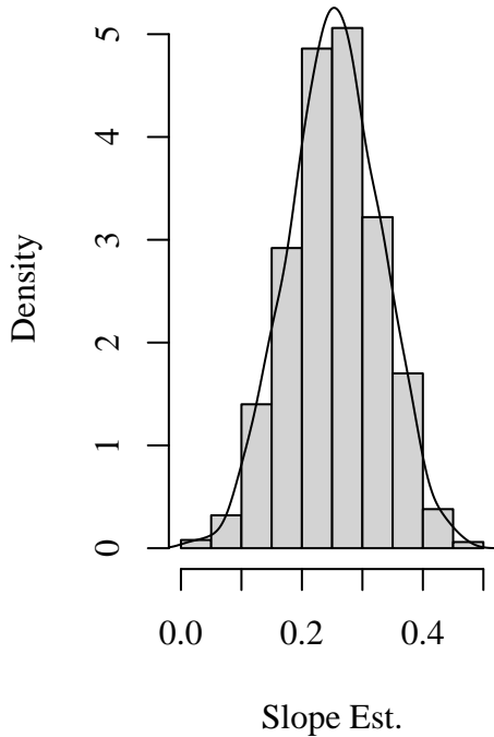
Heteroskedastic Data
