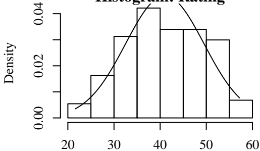
Histogram: Rating
