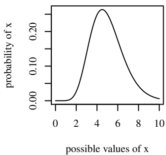
shape=10,scale=0.5
