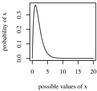
shape=2,scale=1
