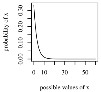
shape=1,scale=3
