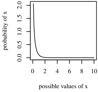
shape=0.5,scale=0.5
