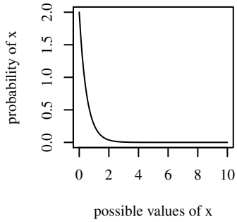
shape=1,scale=0.5
