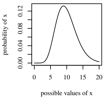
shape=10,scale=1
