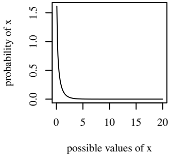
shape=0.5,scale=1
