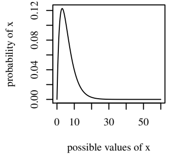
shape=2,scale=3
