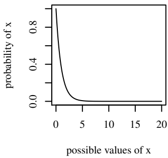
shape=1,scale=1
