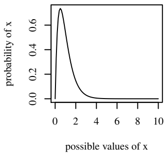
shape=2,scale=0.5
