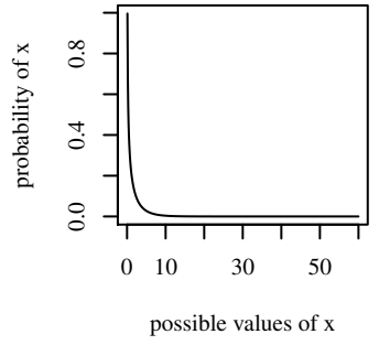
shape=0.5,scale=3
