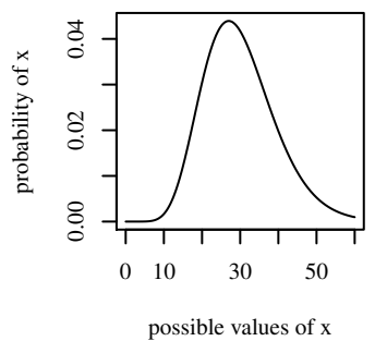
shape=10,scale=3
