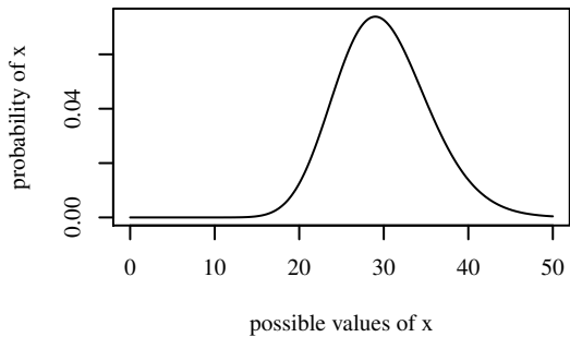
Gamma(shape=30,scale=1,)
