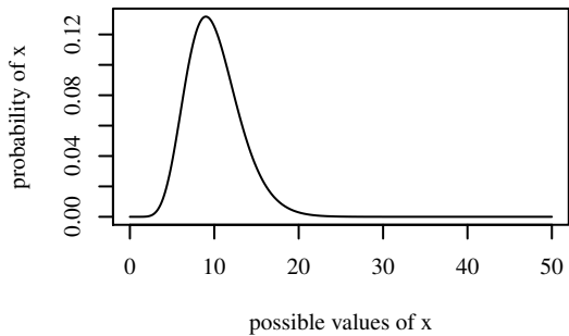
Gamma(shape=10,scale=1,)
