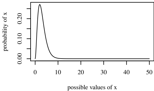
Gamma(shape=3,scale=1,)
