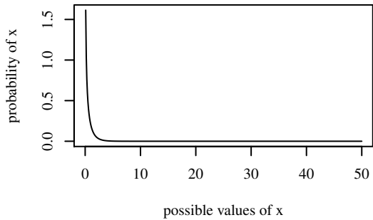
Gamma(shape=0.5,scale=1,)
