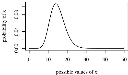
Gamma(shape=15,scale=1,)
