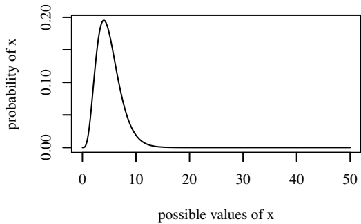
Gamma(shape=5,scale=1,)
