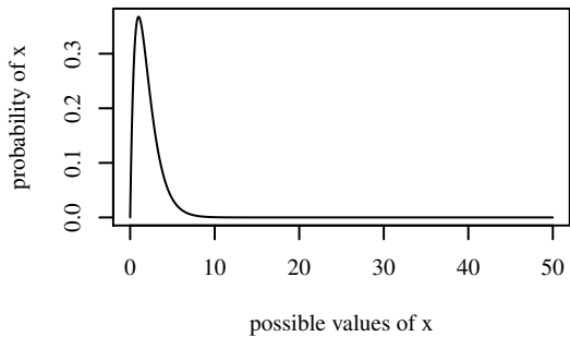
Gamma(shape=2,scale=1,)
