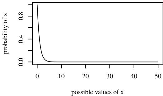
Gamma(shape=1,scale=1,)
