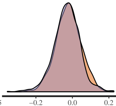
Sentiment^2
