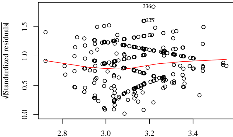
Scale-Location
