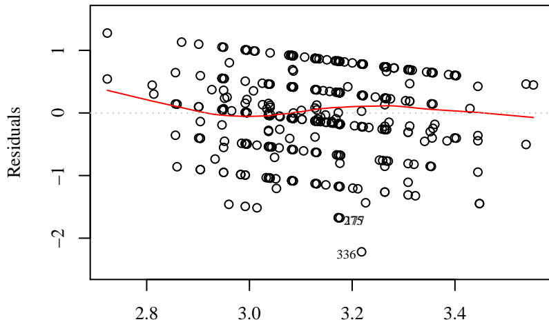
Residuals vs Fitted
