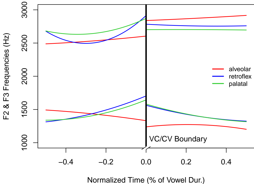
Modal aCa formant transitions in most distinct speaker (M06)
