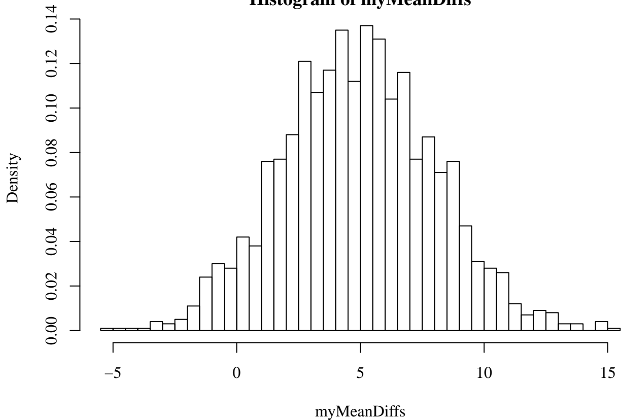
Histogram of myMeanDiffs
