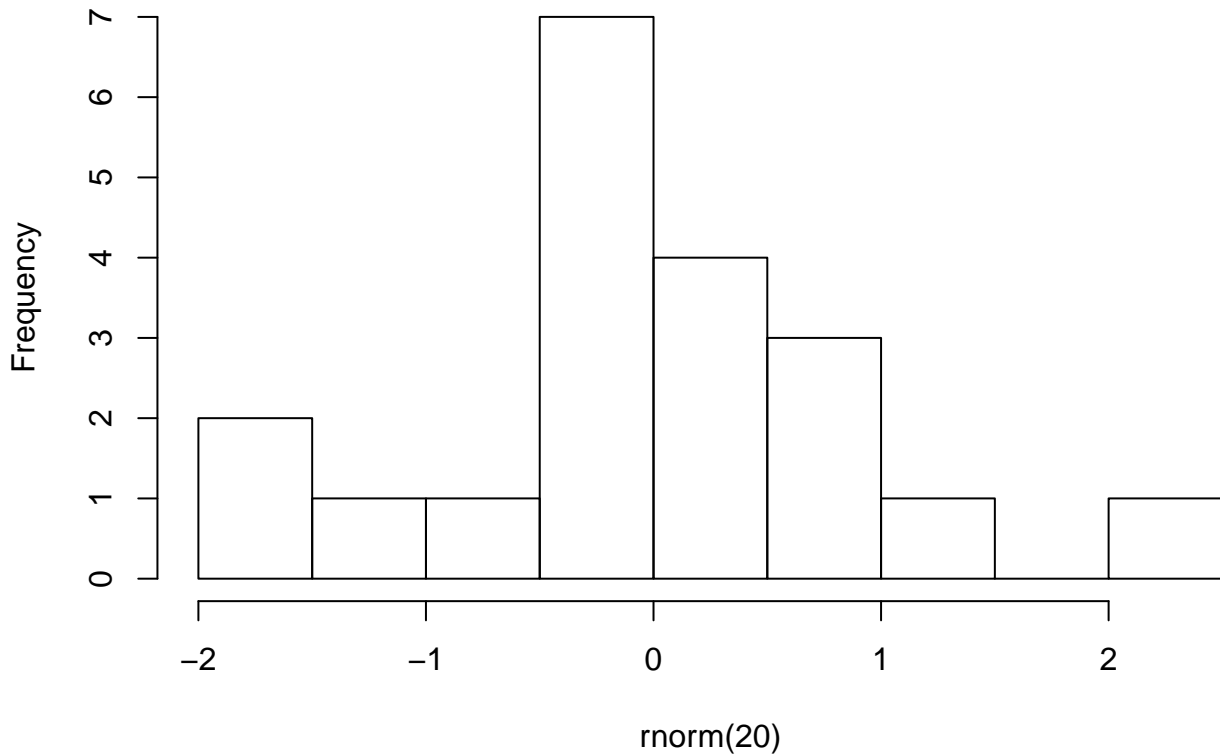
Histogram of rnorm(20)
