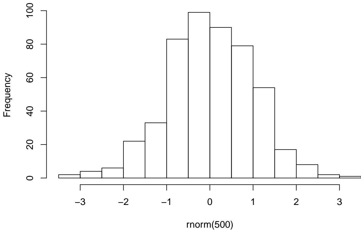
Histogram of rnorm(500)
