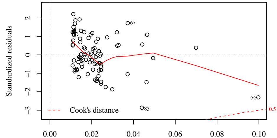
Residuals vs Leverage
