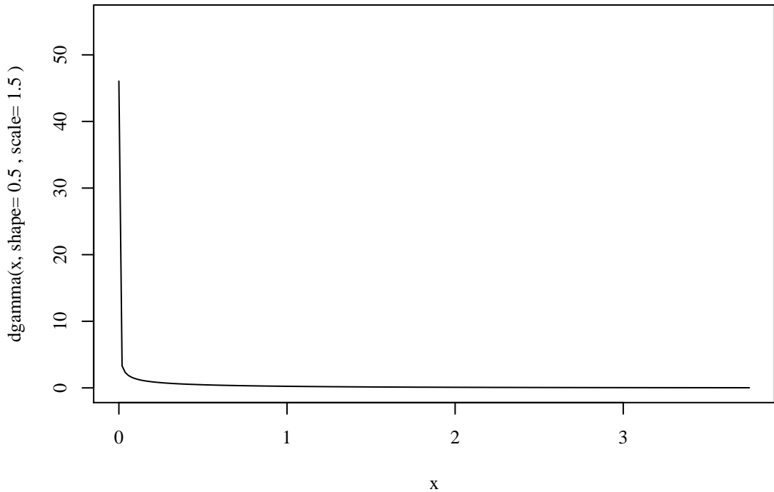
PDF of Gamma( 0.5 , 1.5 )
