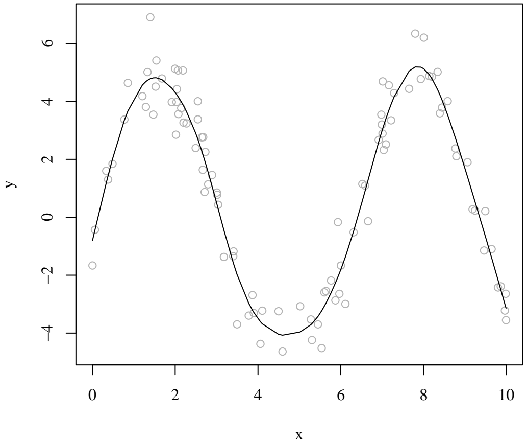
pspline with CV selection of smooth parameter
