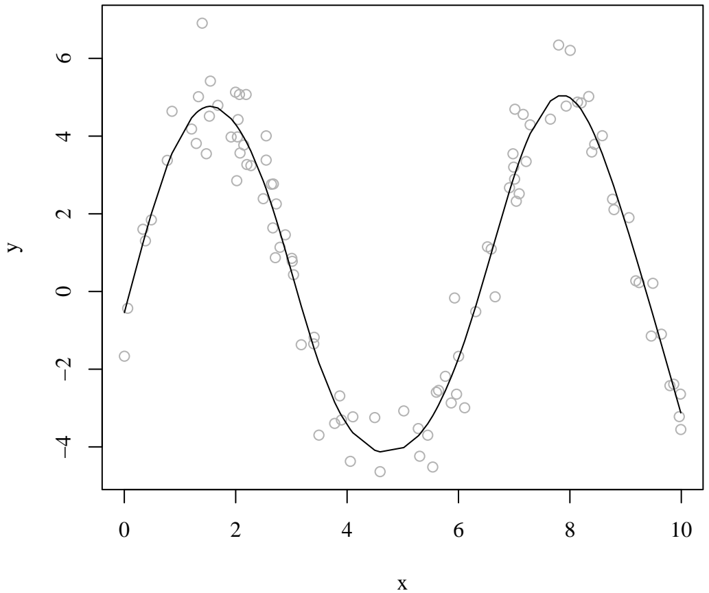
pspline method=2, df=10
