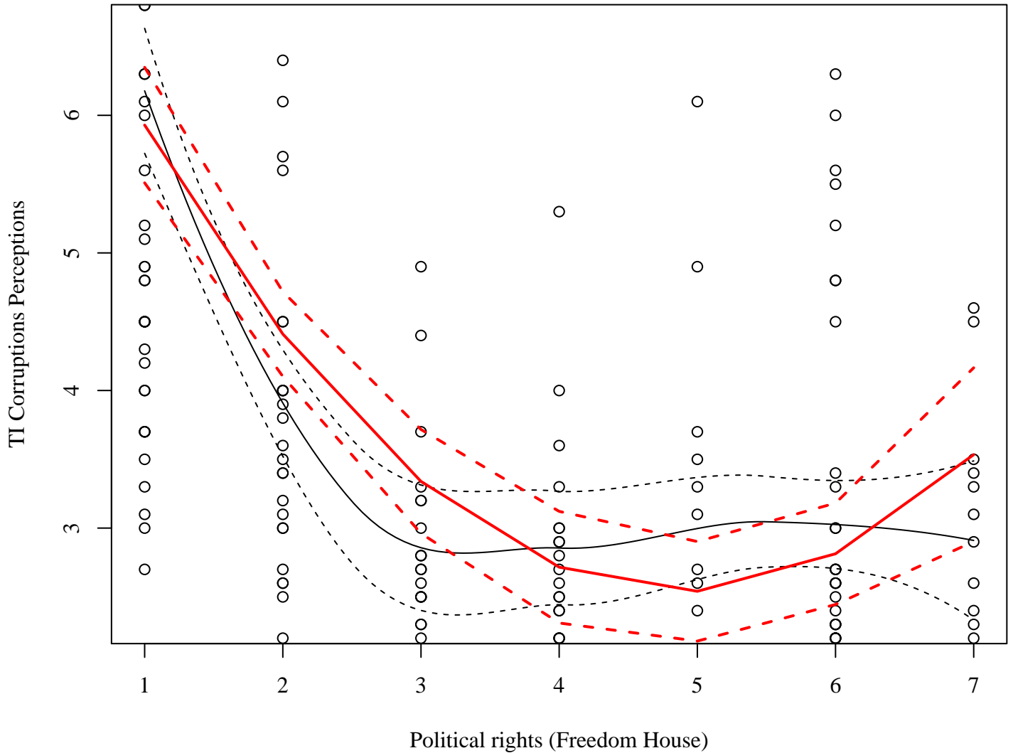
Locfit(nn=0.75) with Confidence Intervals
