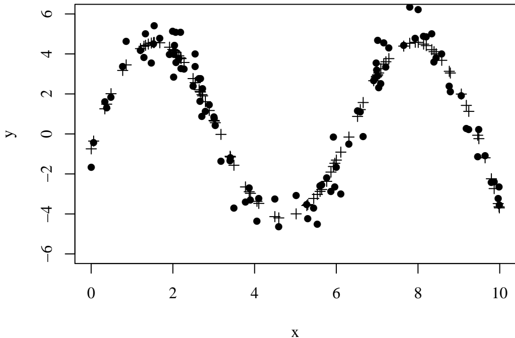
loess output from MASS without deceptive line
