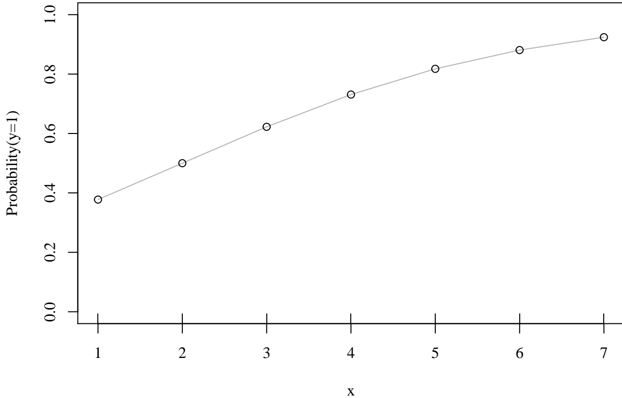
The True Model, \beta_0 = -1 , \beta_1 = 0.5
