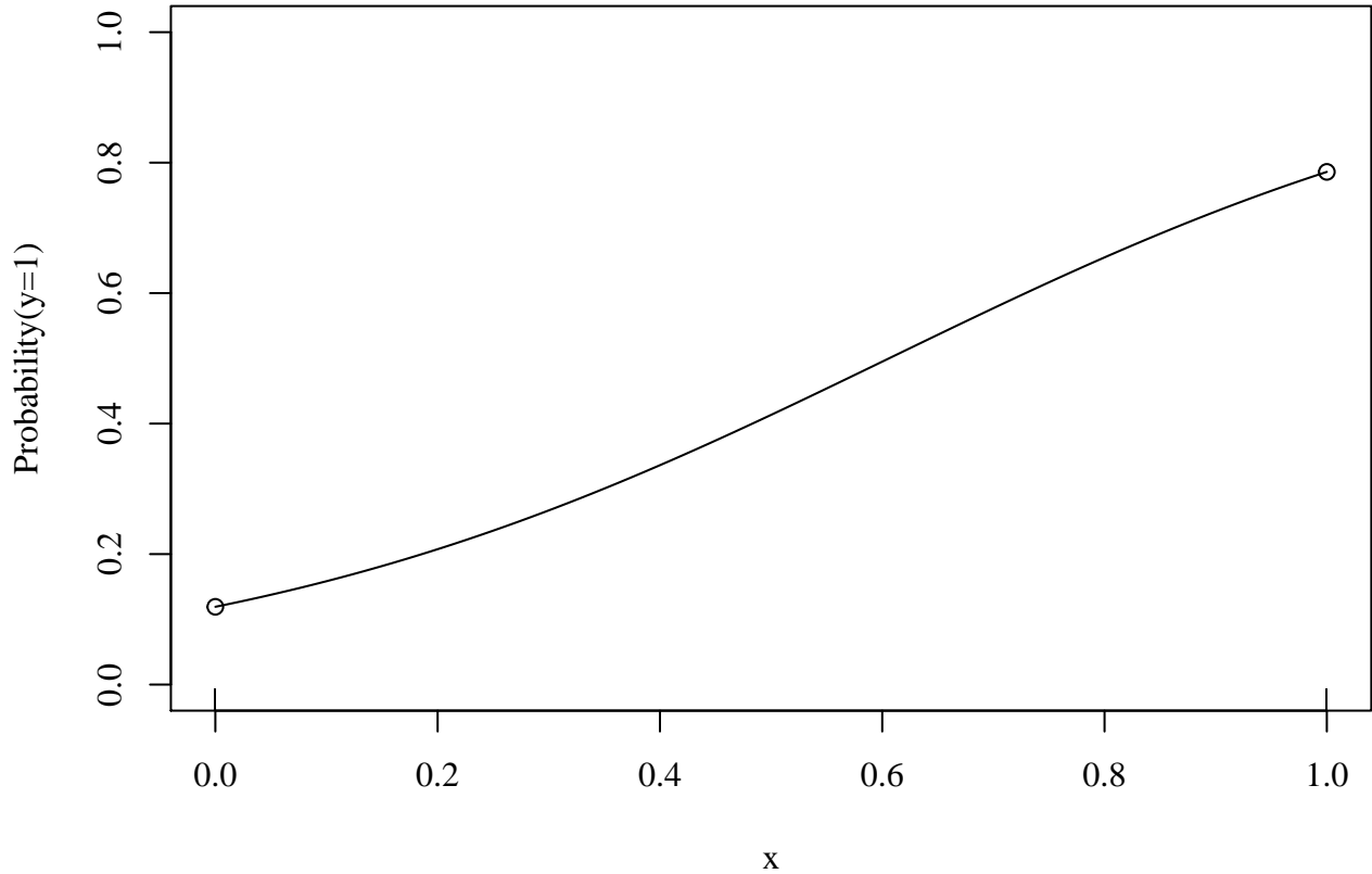
The True Model, beta0 = -2 , beta1 = 3.3
