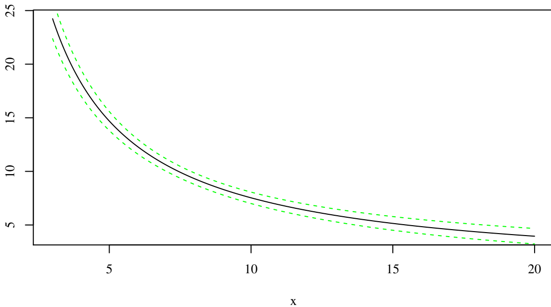
Gaussian, link=identity
