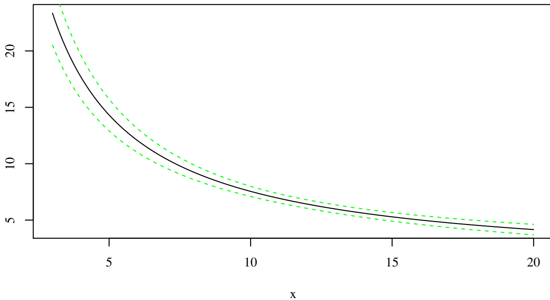
Gamma, link=identity
