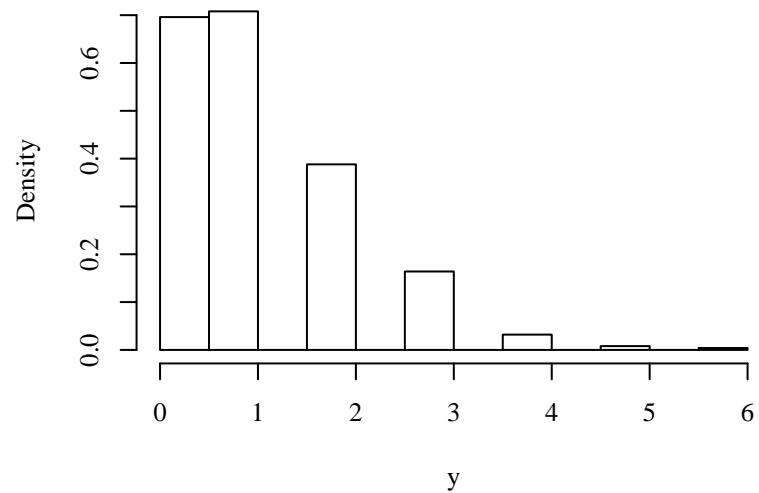
lambda=1.0
