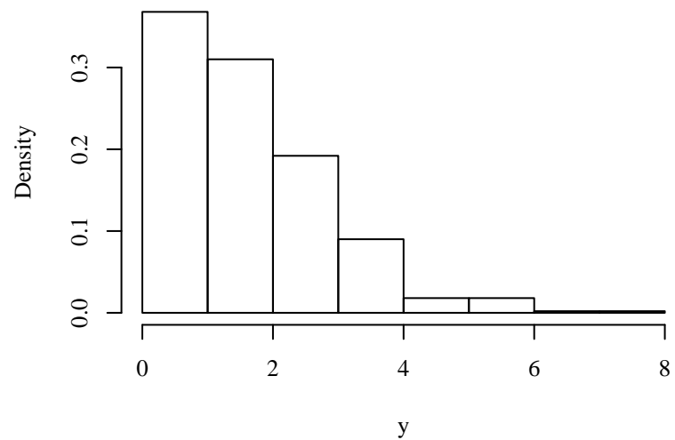
lambda=2.0
