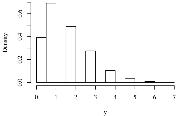
lambda=1.5
