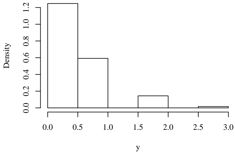
lambda=0.5
