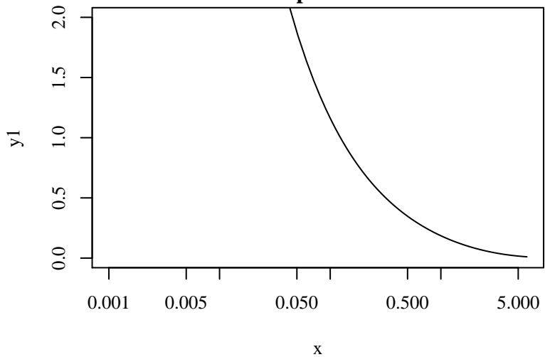
shape = 1/3
