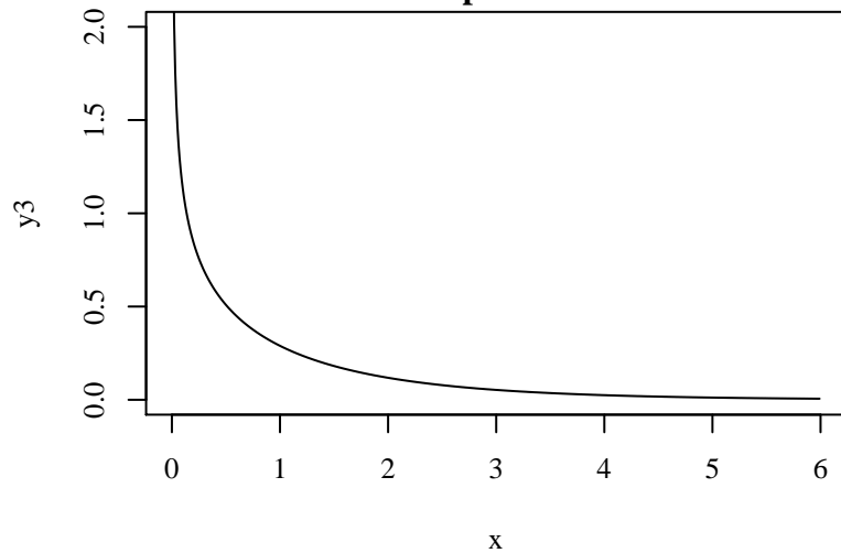
shape = 3/2
