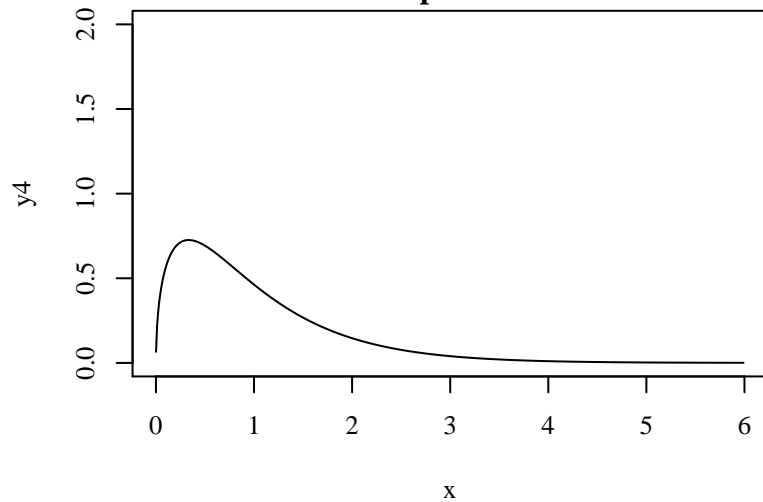
shape = 1.5
