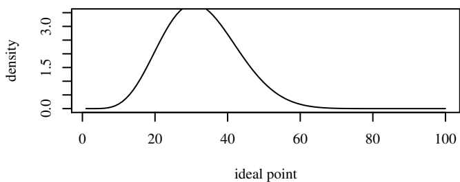
Beta(6.34, 13.47) mode=0.3 mean=0.32, var=0.01
