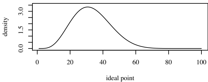
Beta(5.03, 10.41) mode=0.3 mean=0.33, var=0.013
