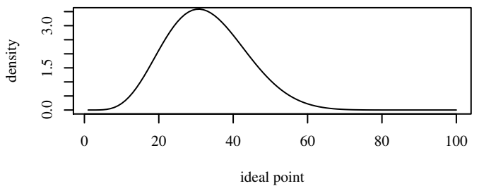
Beta(5.69, 11.94) mode=0.3 mean=0.32, var=0.012
