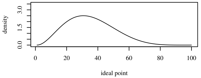
Beta(3.07, 5.82) mode=0.3 mean=0.34, var=0.023
