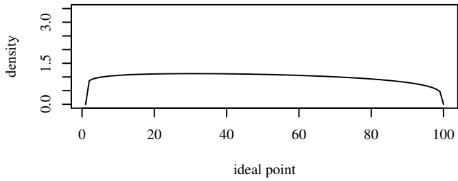
Beta(1.1, 1.23) mode=0.3 mean=0.47, var=0.075
