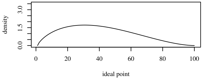
Beta(1.76, 2.76) mode=0.3 mean=0.39, var=0.043
