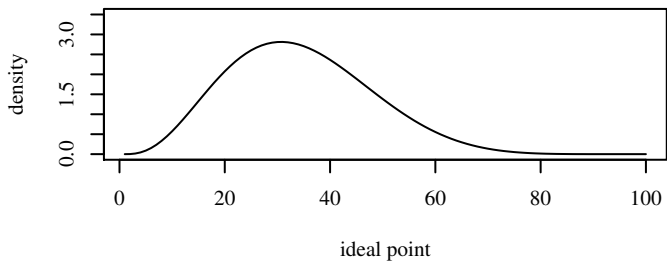
Beta(3.72, 7.35) mode=0.3 mean=0.34, var=0.018
