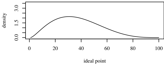
Beta(2.41, 4.29) mode=0.3 mean=0.36, var=0.03
