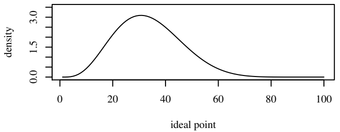
Beta(4.38, 8.88) mode=0.3 mean=0.33, var=0.016
