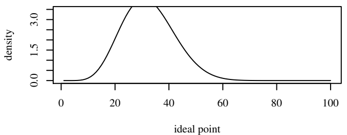
Beta(7, 15) mode=0.3 mean=0.32, var=0.009
