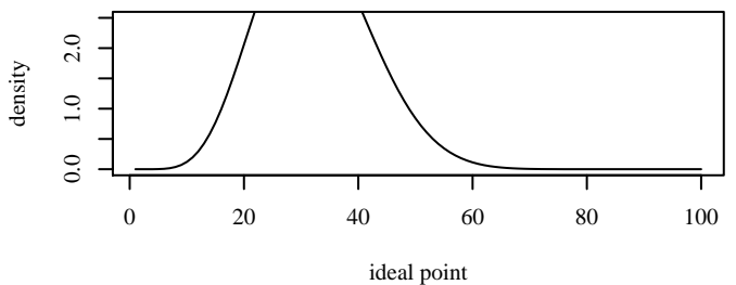
Beta(7, 15) mode=0.3 mean=0.32, var=0.009
