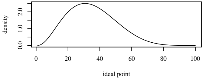
Beta(3.07, 5.82) mode=0.3 mean=0.34, var=0.023
