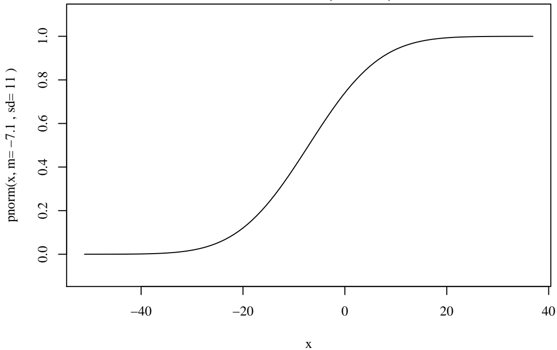
CDF of Normal( -7.1, 11^2 )
