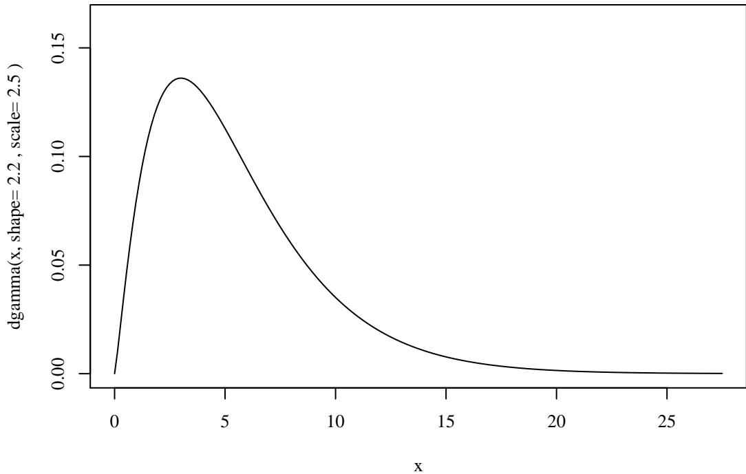
PDF of Gamma( 2.2 , 2.5 )
