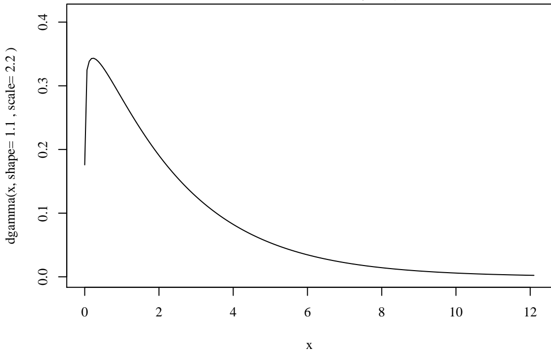
PDF of Gamma( 1.1 , 2.2 )
