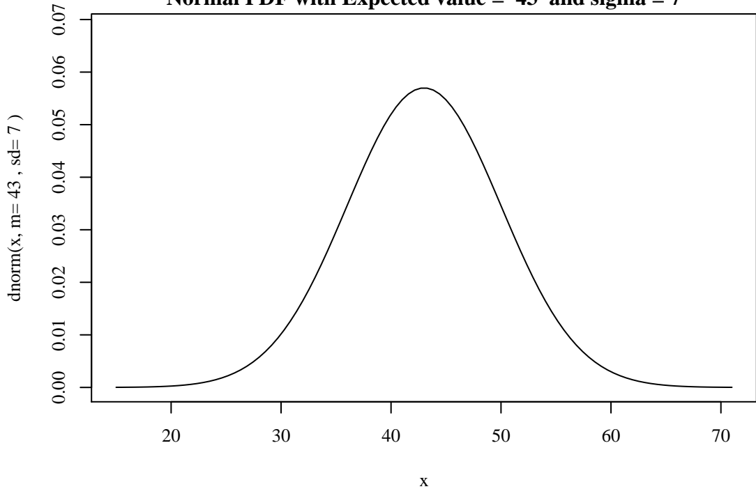
Normal PDF with Expected value = 43 and sigma = 7
